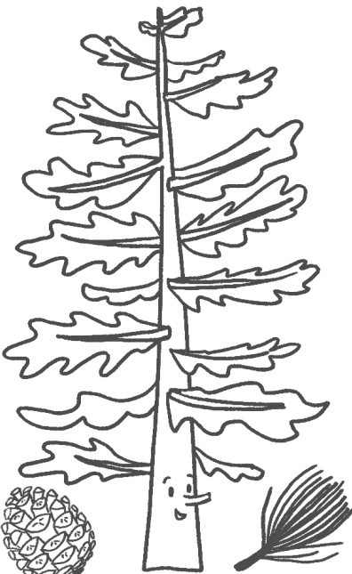
White Pine
