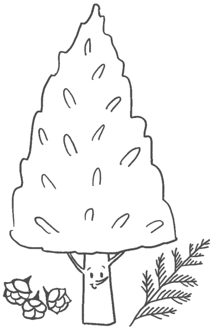
Lawson Cypress
